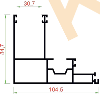
TG-103 YAN KASA (ALT) 1.169 KG/M
