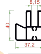
TGT-106 KENET (TEK CAM) 0.913 KG/M
